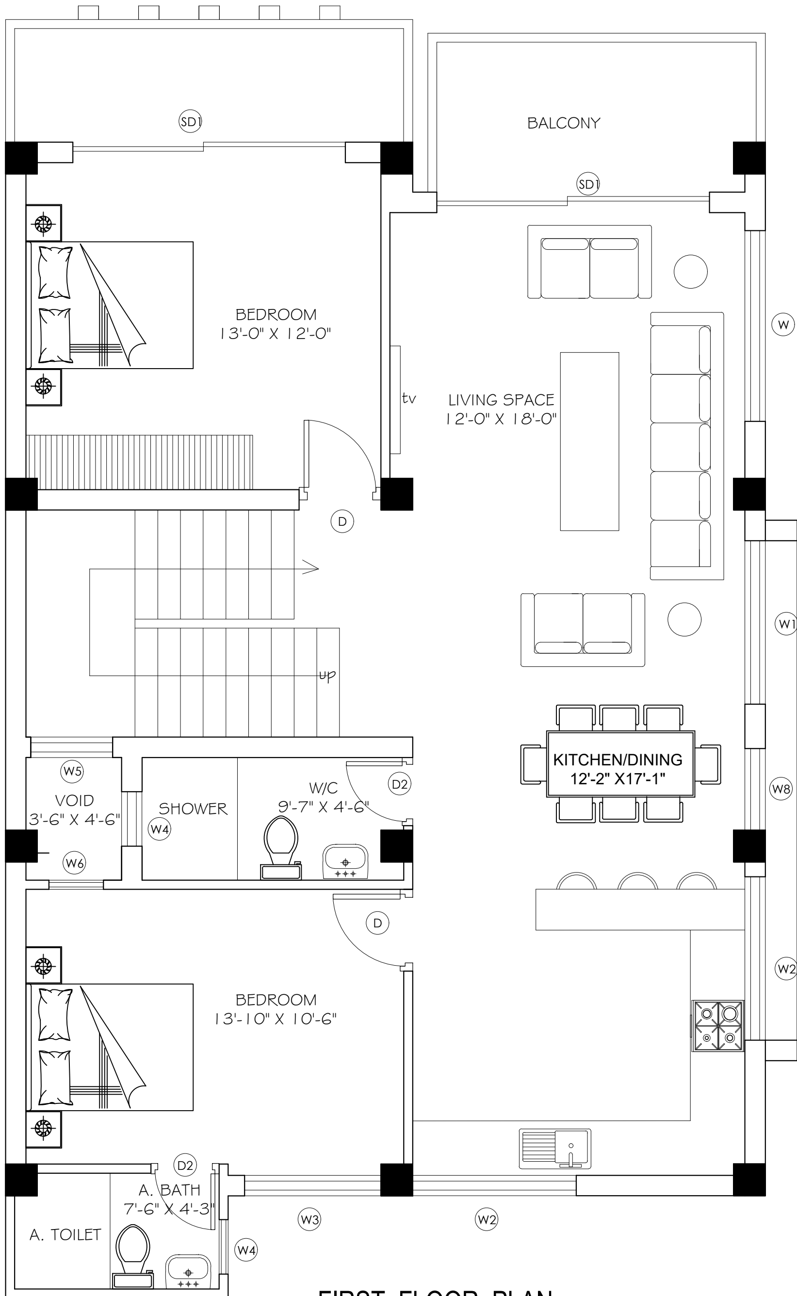
FIRST FLOOR PLAN FOR COUNTABLE AREA:-1108.43 SQ.FT. FOR NON COUNTABLE AREA:-116.75 SQ.FT TOTAL AREA:-1225.18 SQ.FT.
